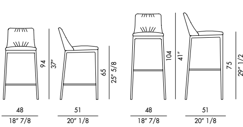
MAX STOOL DELUXE_base legno / wood base Design Antoy Filips
