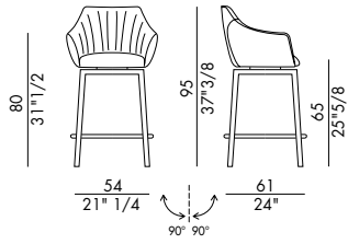
JANE STOOL_4 gambe metallo / 4 metal legs Design Antoy Filips
