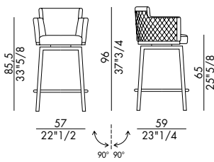
ELY STOOL DIAMOND_4 gambe metallo / 4 metal legs Design Assmann+ Kleene GbR
