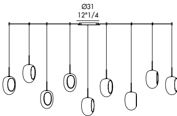
FOS_9 sospensione (per piano 460 cm) pendant (for top 460 cm)
