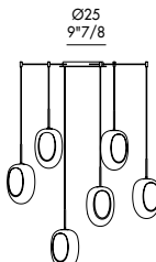
FOS_6 sospensione (per piano Ø 220 cm) pendant (for top Ø 220 cm)
